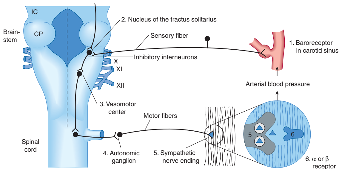
FIGURE 11–2 Baroreceptor reflex arc.
