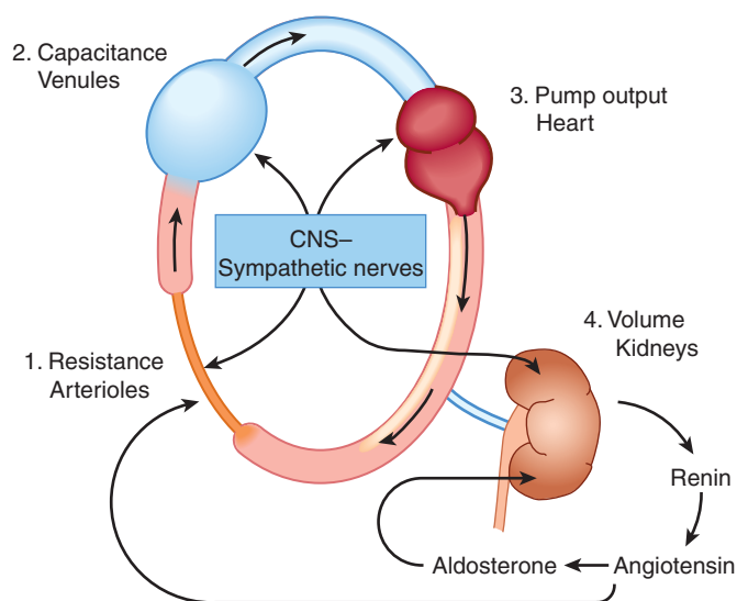
FIGURE 11–1 Anatomic sites of blood pressure control.
